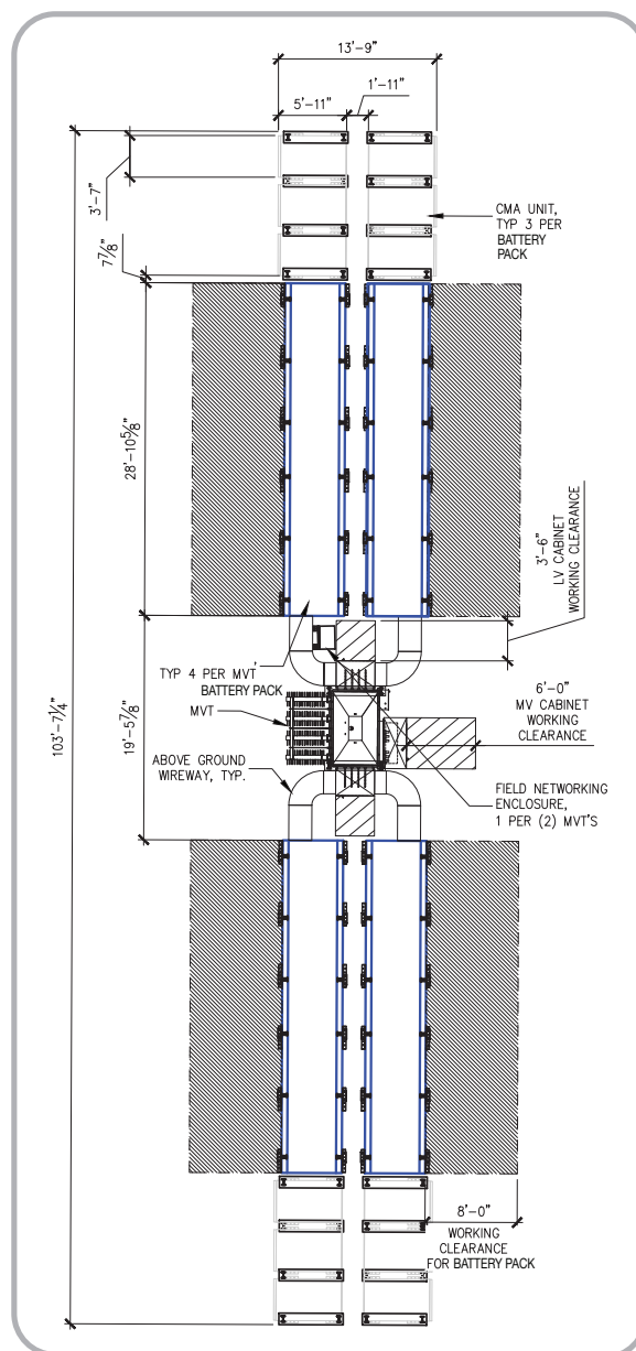
Typical Power Block
